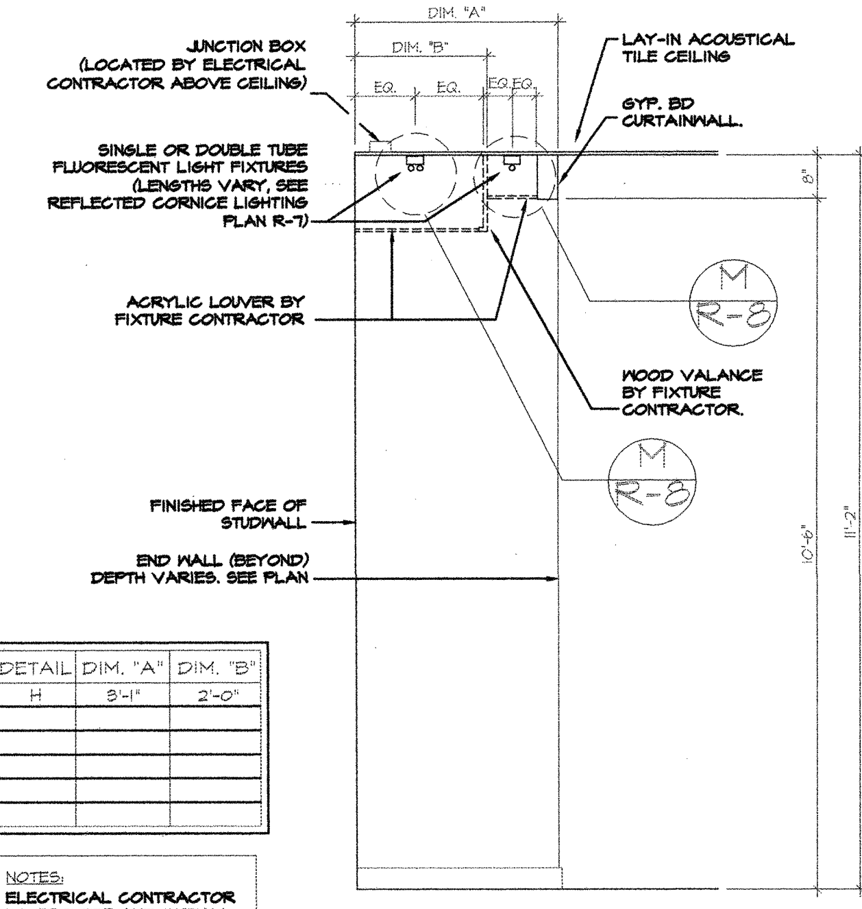
I LIGHTING SECTION SCALE: 1/2" = 1'-0"
