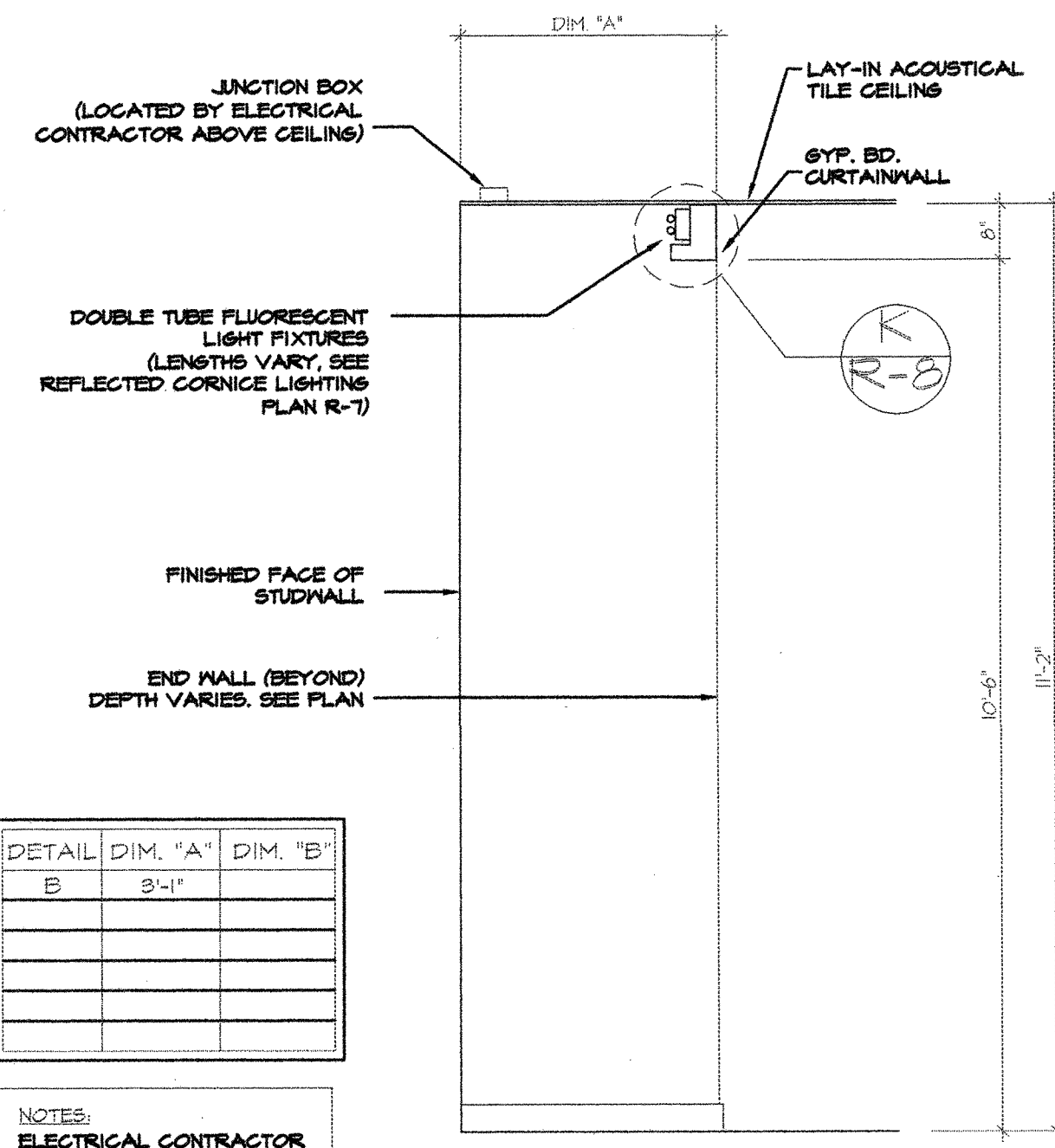
B LIGHTING SECTION SCALE: 1/2" = 1'-0"
