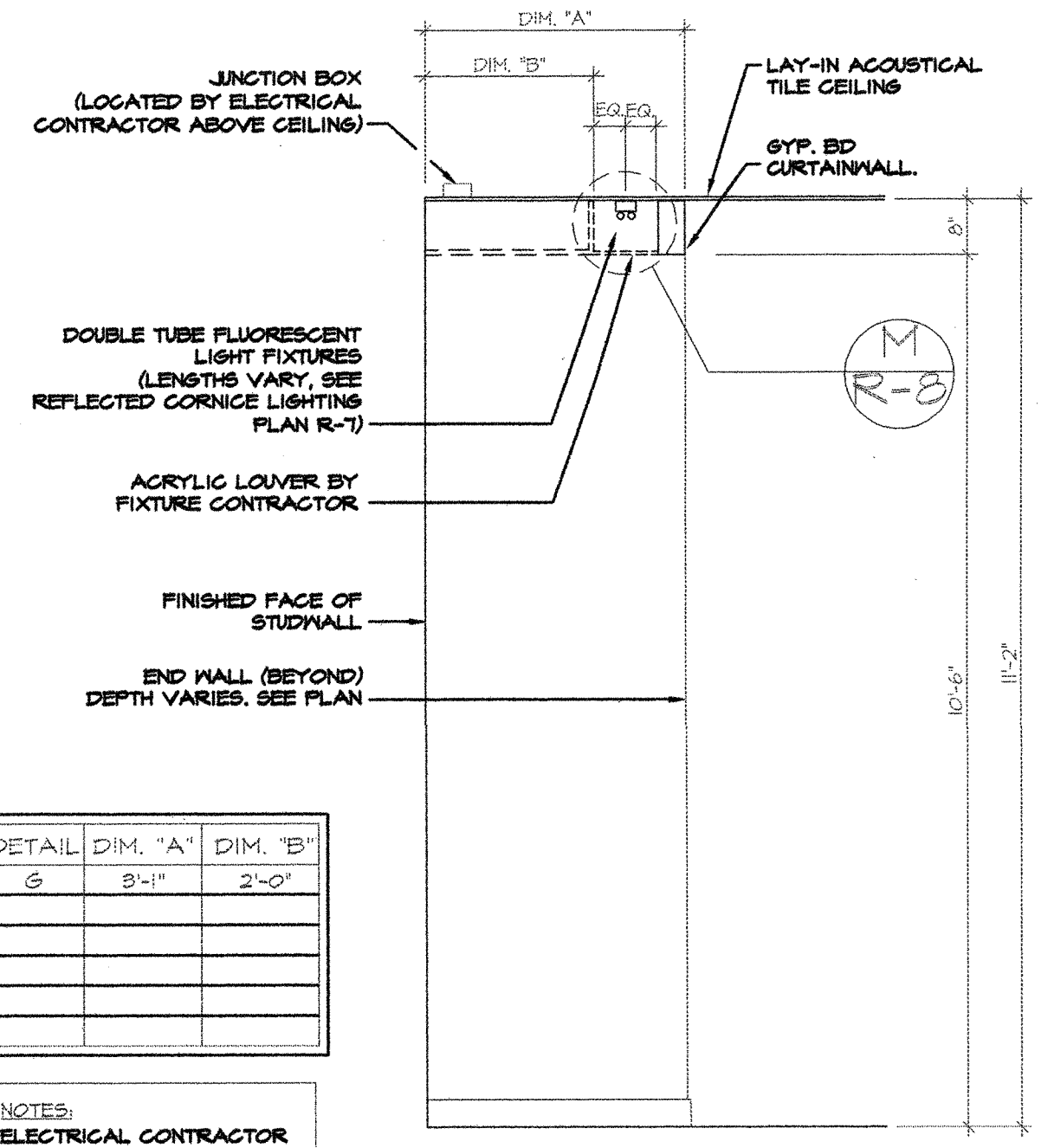
G LIGHTING SECTION SCALE: 1/2" = 1'-0"
