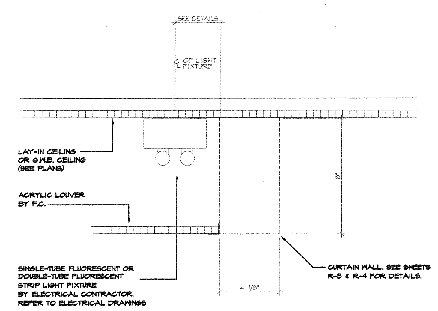
I LIGHTING SECTION SCALE: 1/2" = 1'-0"
