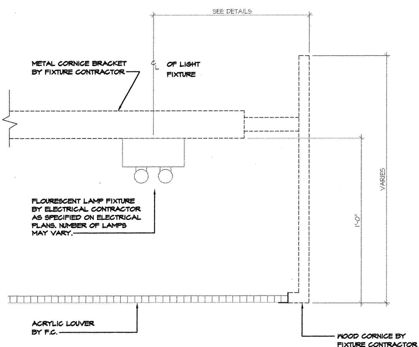
G LIGHTING SECTION SCALE: 1/2" = 1'-0"
