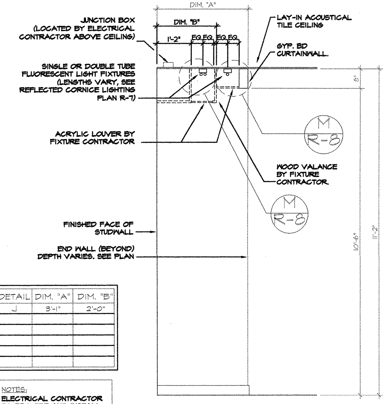
J LIGHTING SECTION SCALE: 1/2" = 1'-0"
