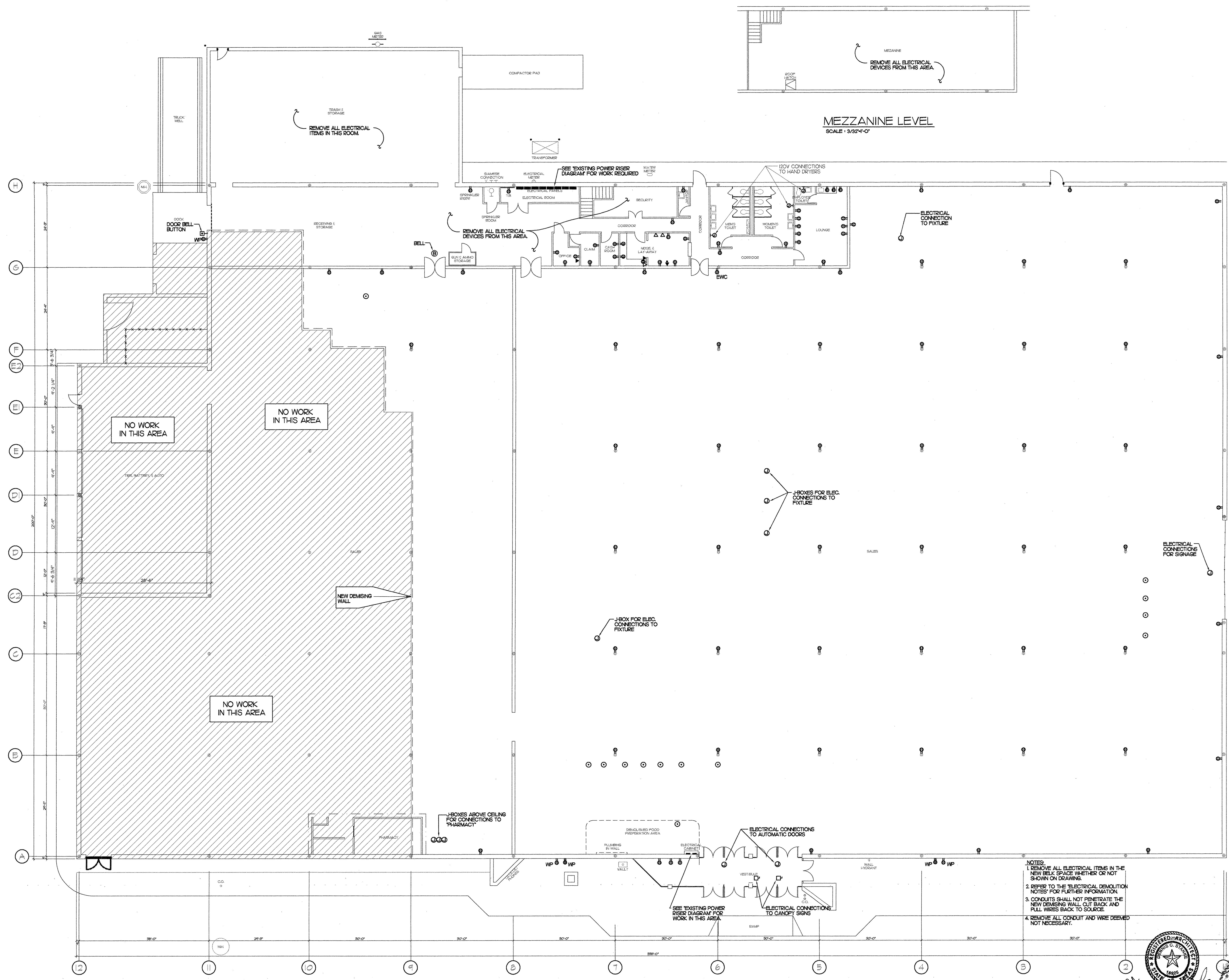
FLOOR ELECTRIC DEMOLITION PLAN SCALE: 3/32"=1'-0"
