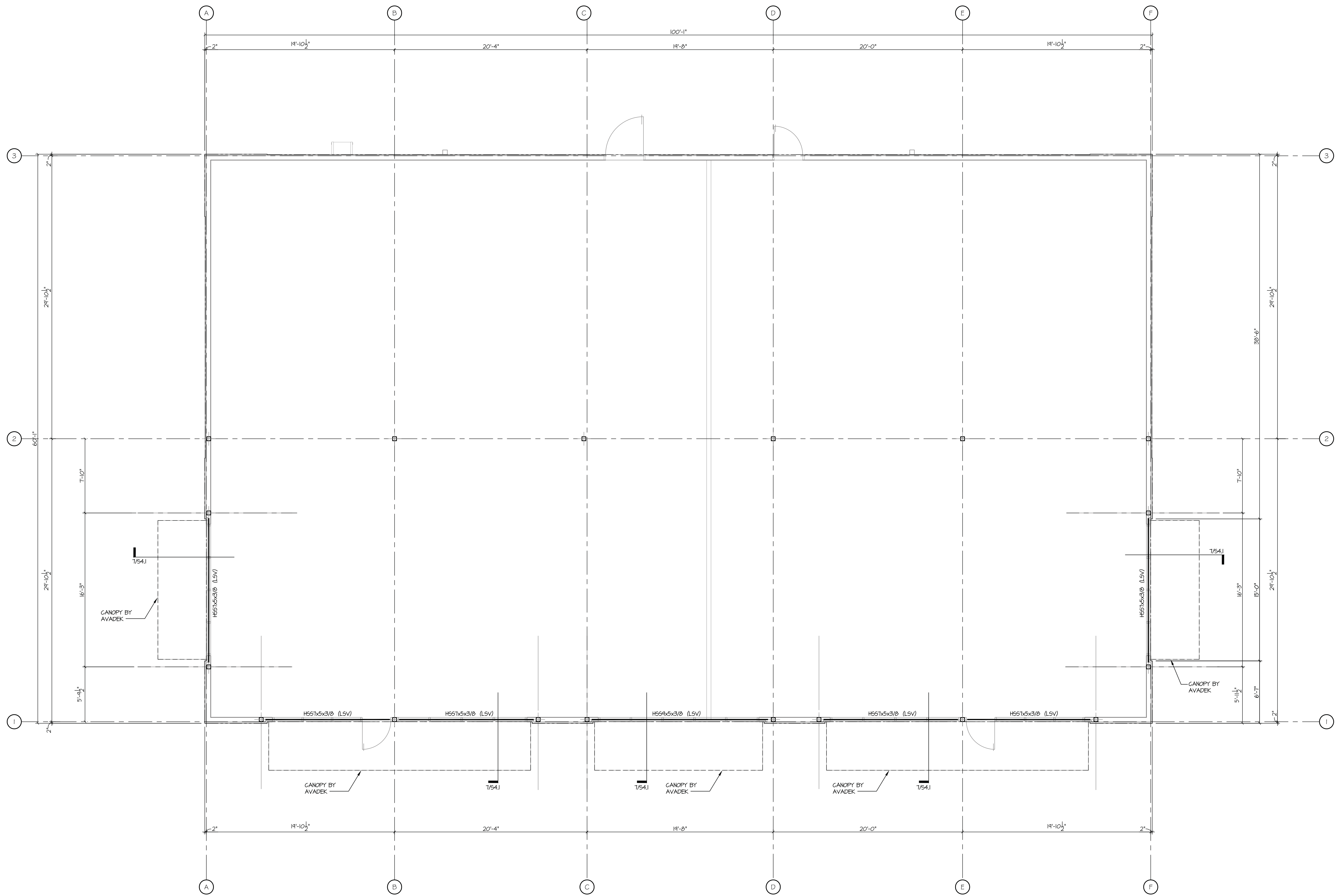
1 CANOPY FRAMING PLAN
