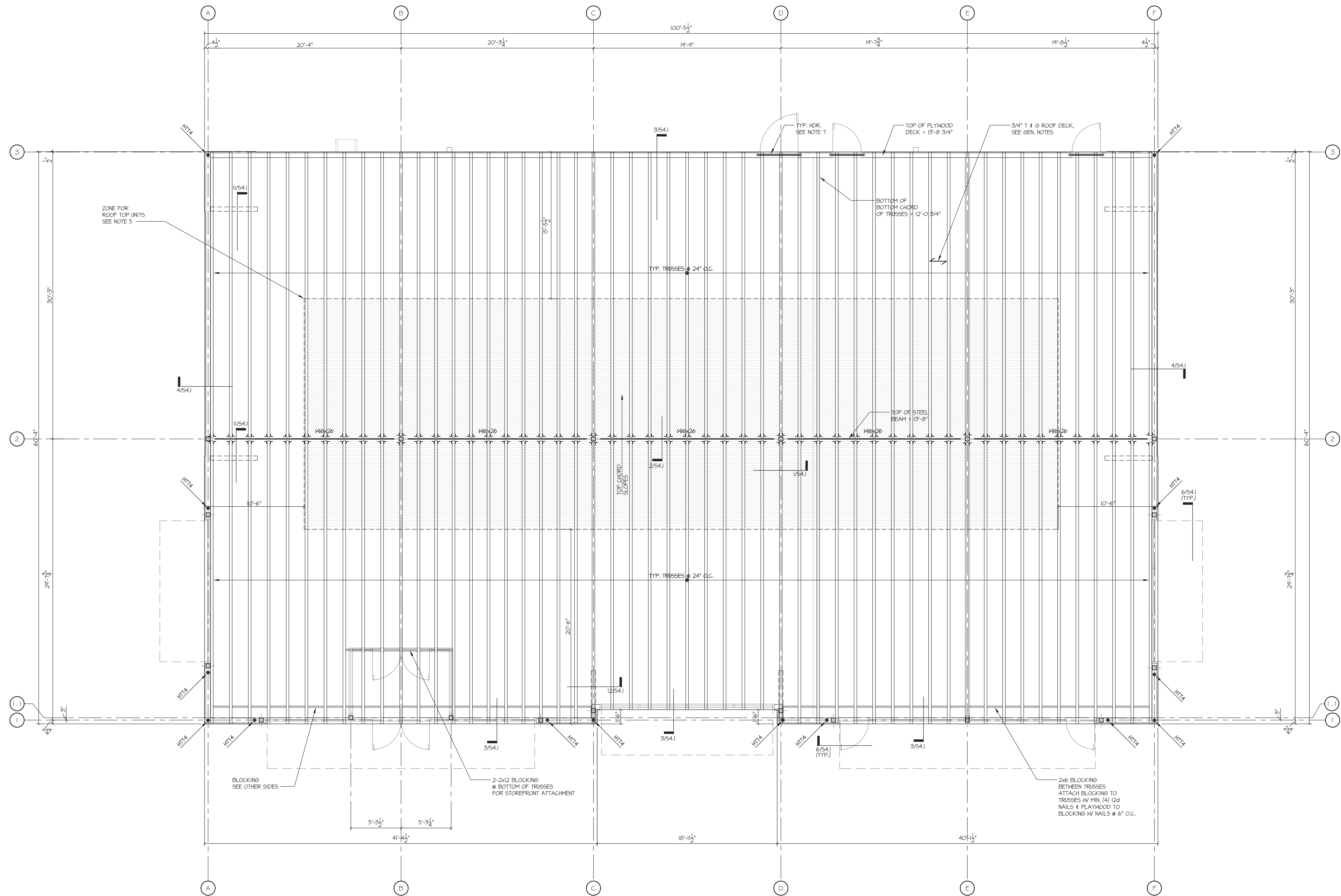
1 ROOF FRAMING PLAN
