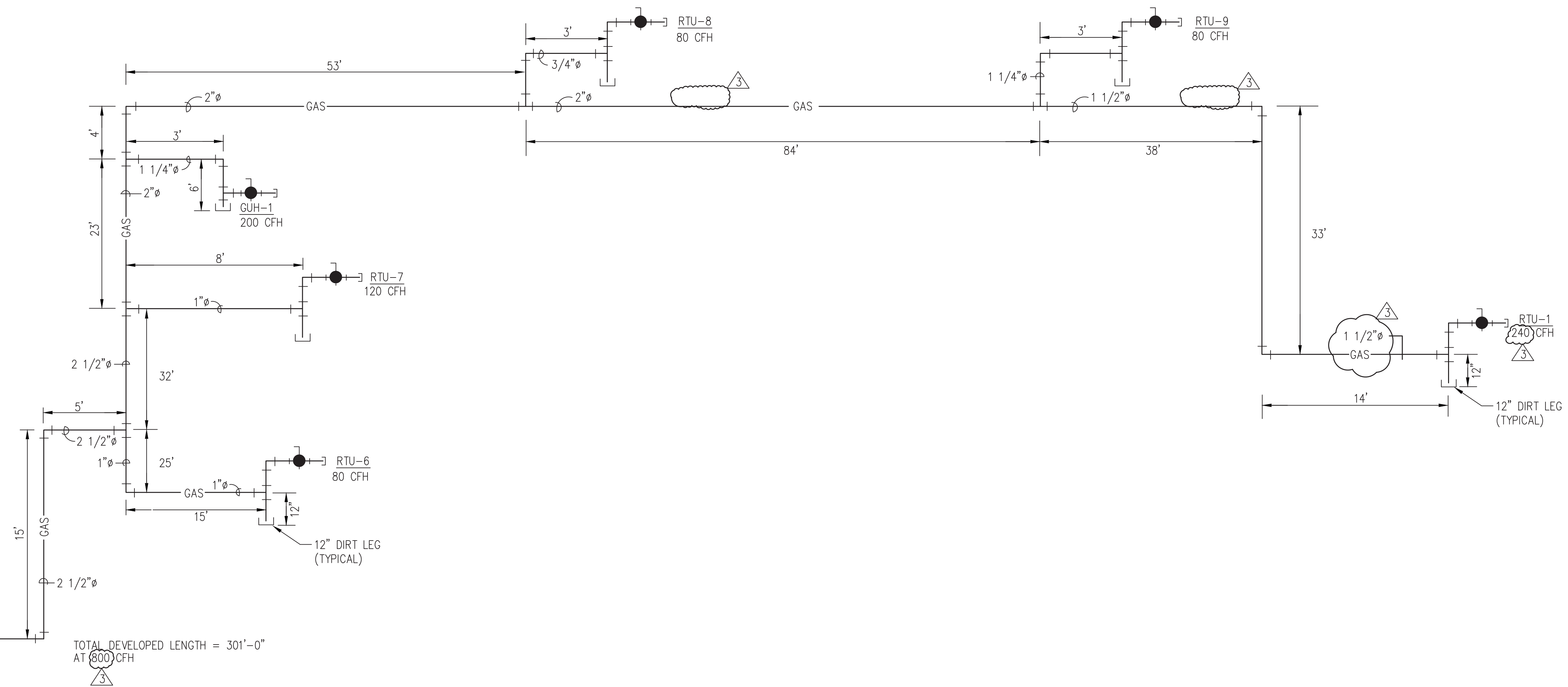
2 GAS PIPING RISER DIAGRAM SCALE: NTS
