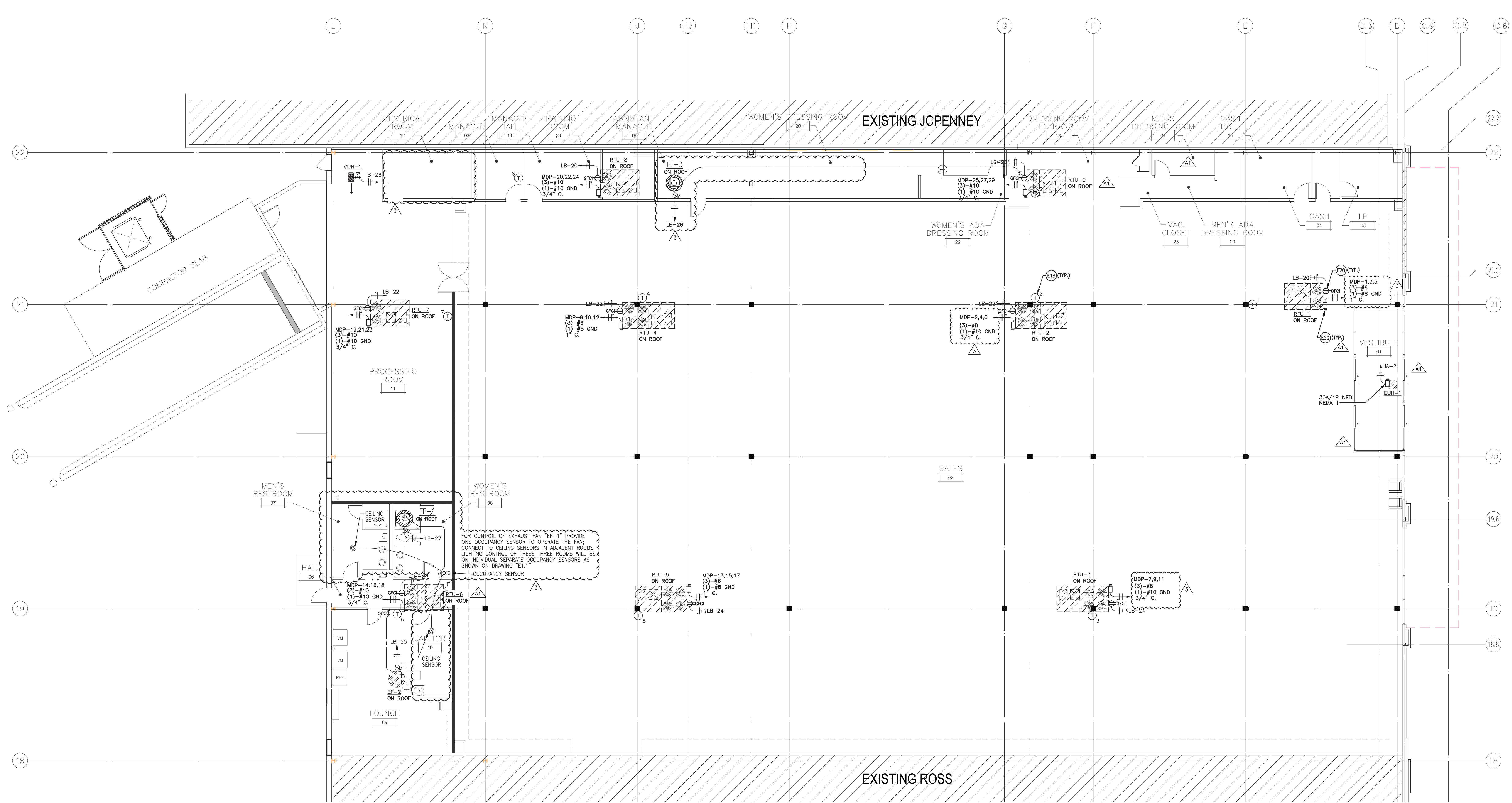
1 ELECTRICAL FLOOR PLAN – MECHANICAL EQUIPMENT E1.4 SCALE: 1/8" = 1'-0"
