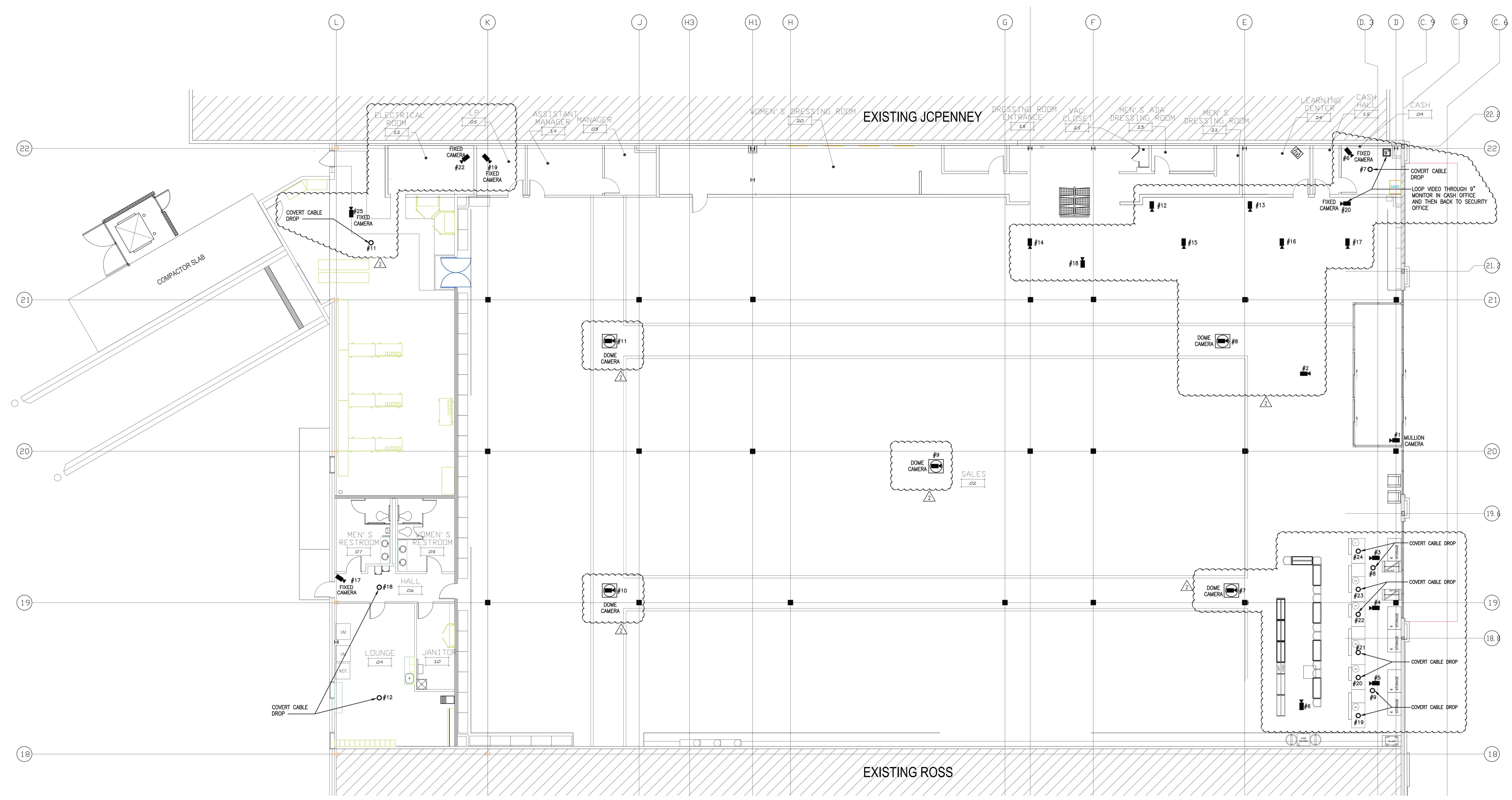
1 SECURITY CAMERAS FLOOR PLAN E1.3 SCALE: 1/8" = 1'-0"
