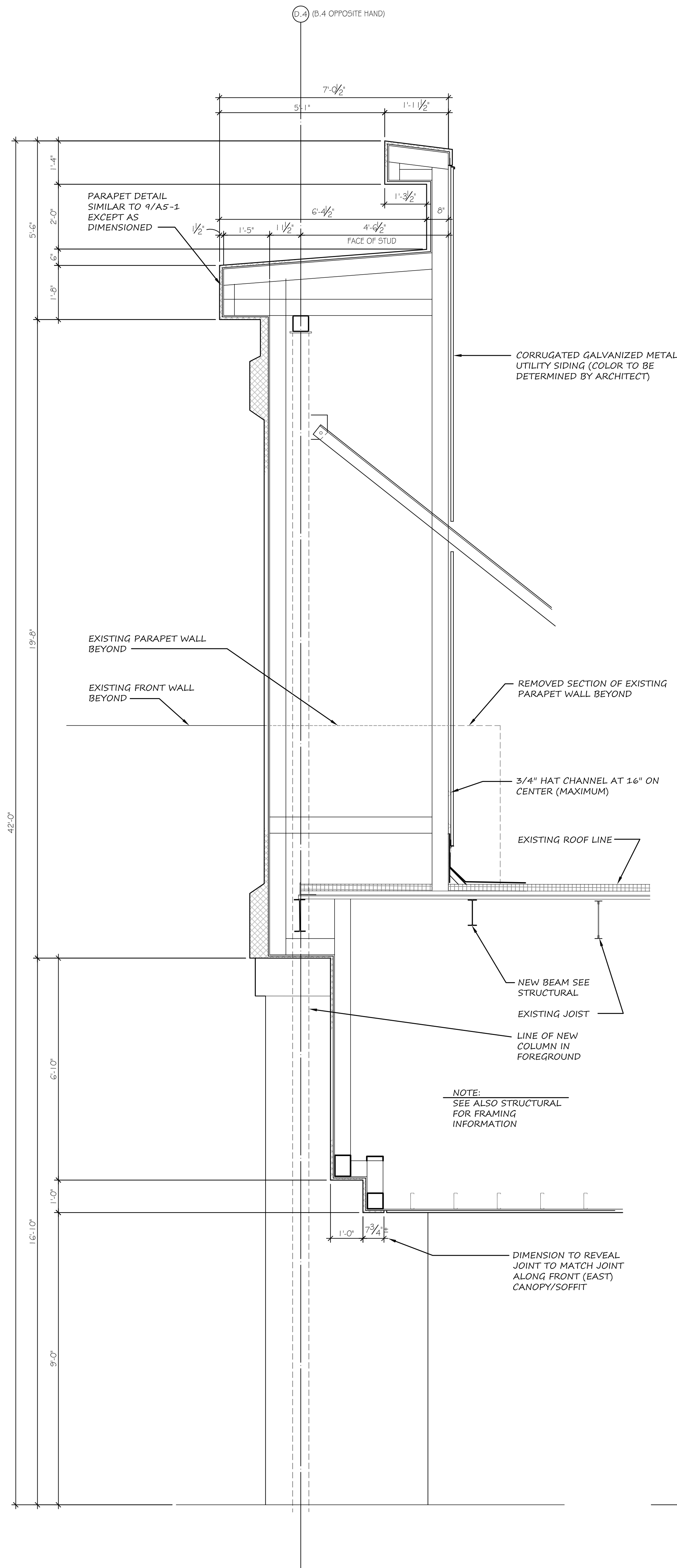
1 | PROPOSED CANOPY RETURN A4-1 | SCALE: 1/2" = 1'-0"
