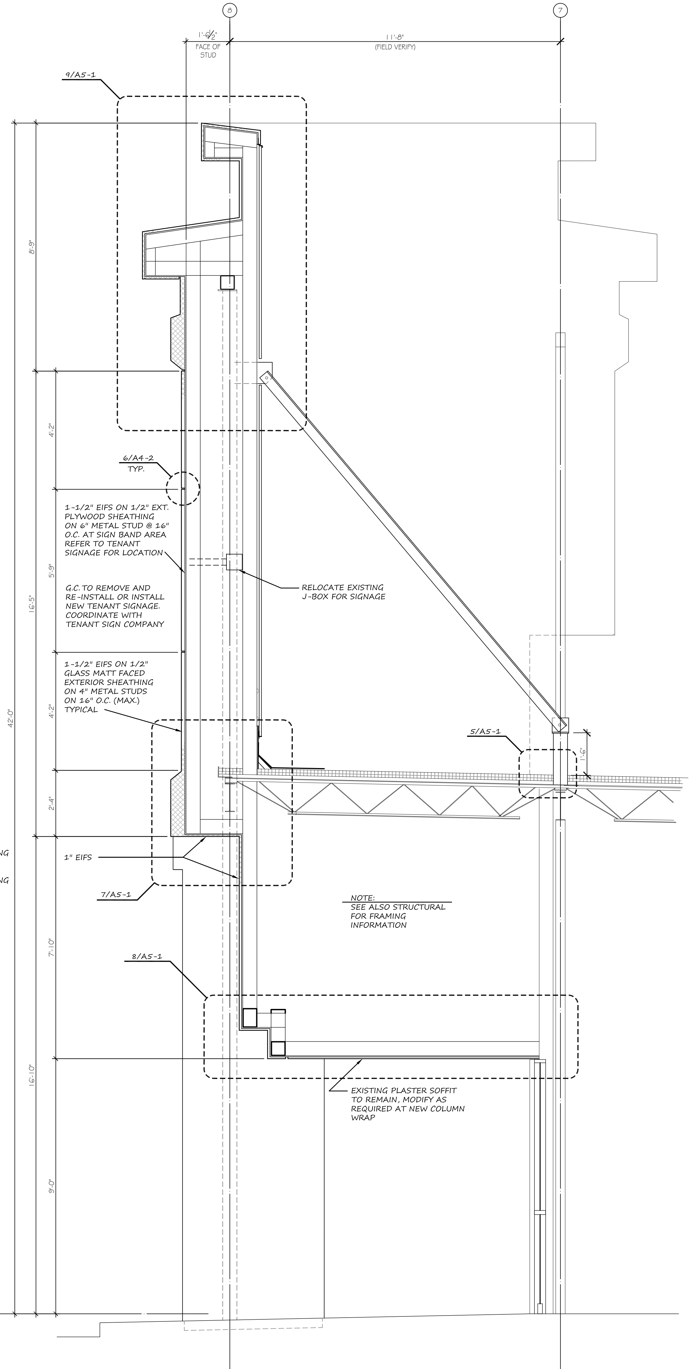
3 | PROPOSED CANOPY SECTION A4-1 | SCALE: 1/2" = 1'-0"
