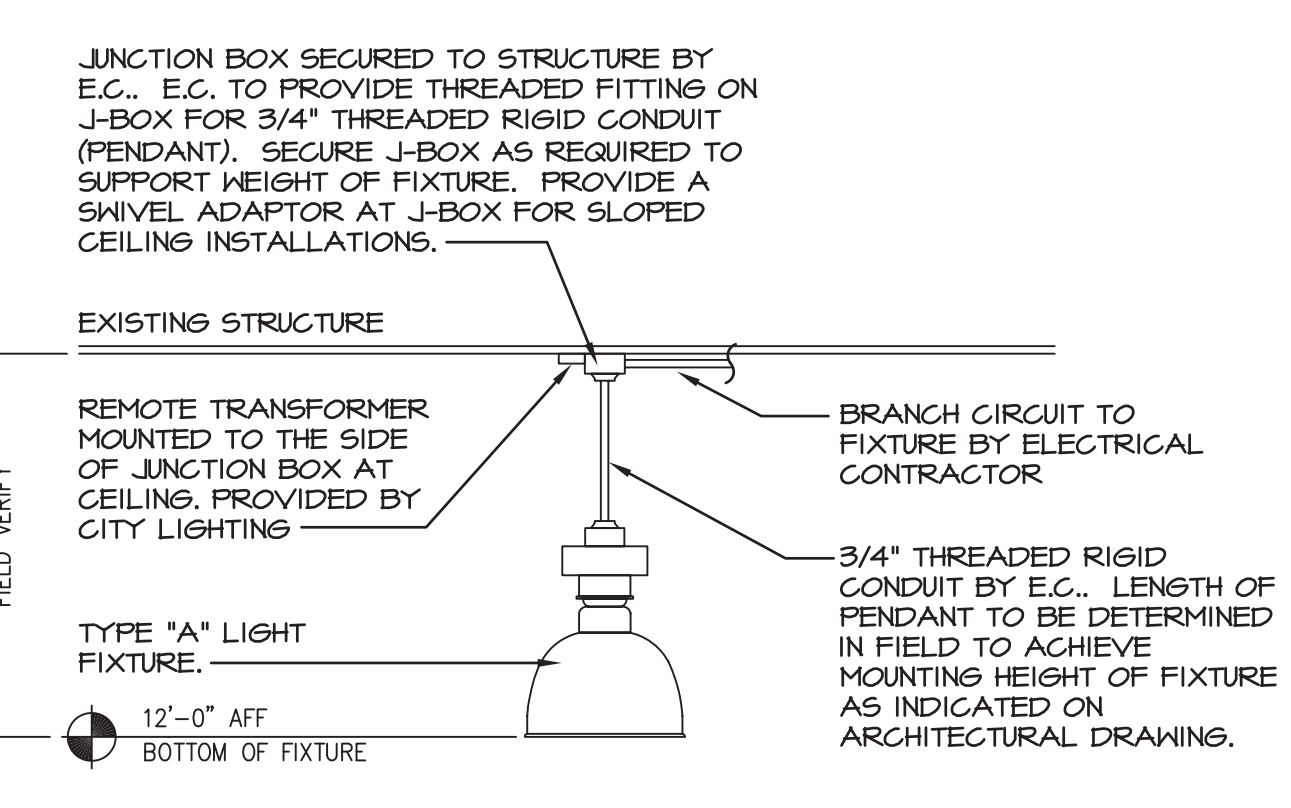
2 DETAIL AT HIGH BAY FIXTURES A8-1 NOT TO SCALE
