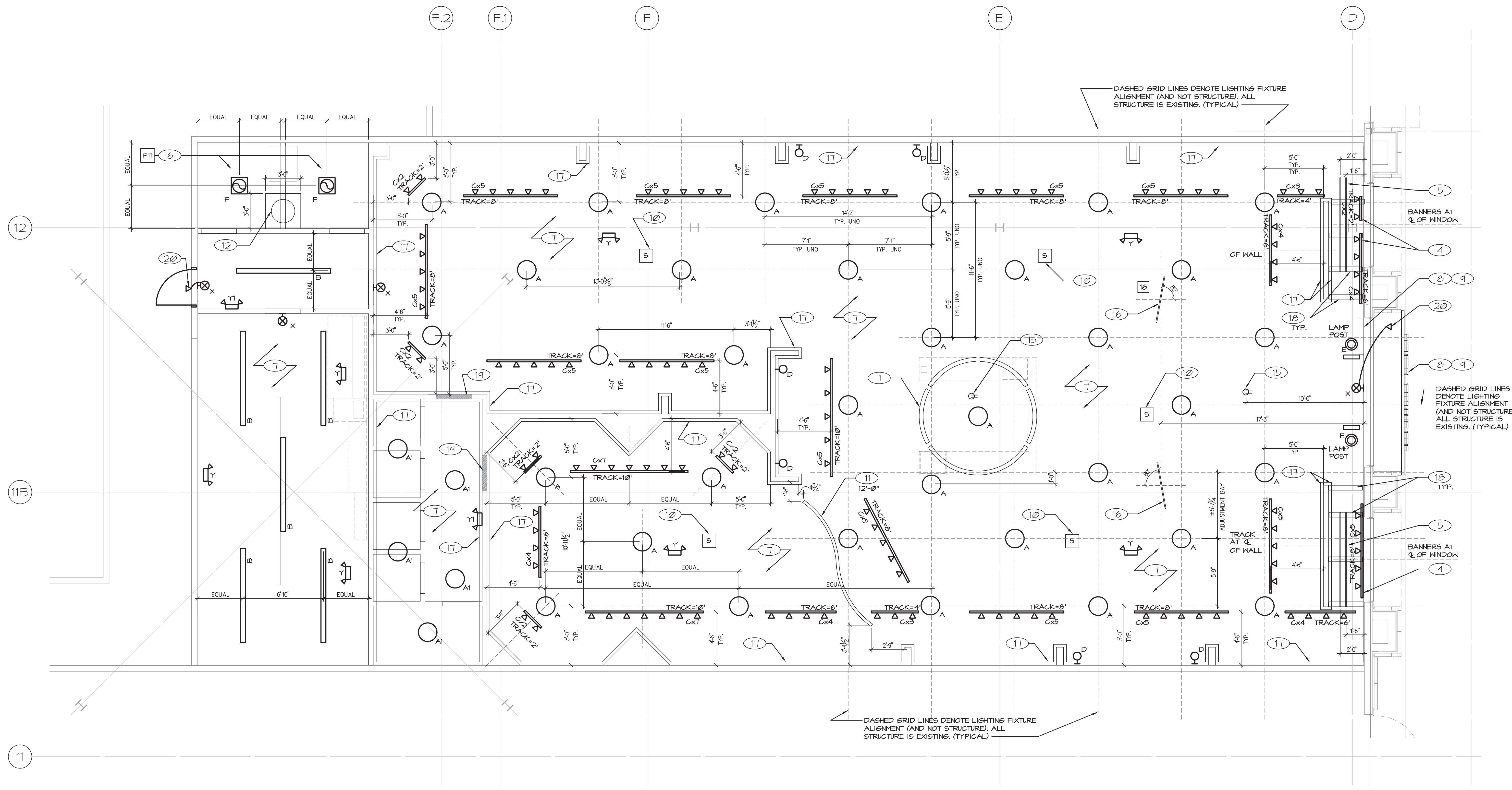
1 REFLECTED CEILING PLAN A8-1 SCALE: 1/4" = 1'-0"
