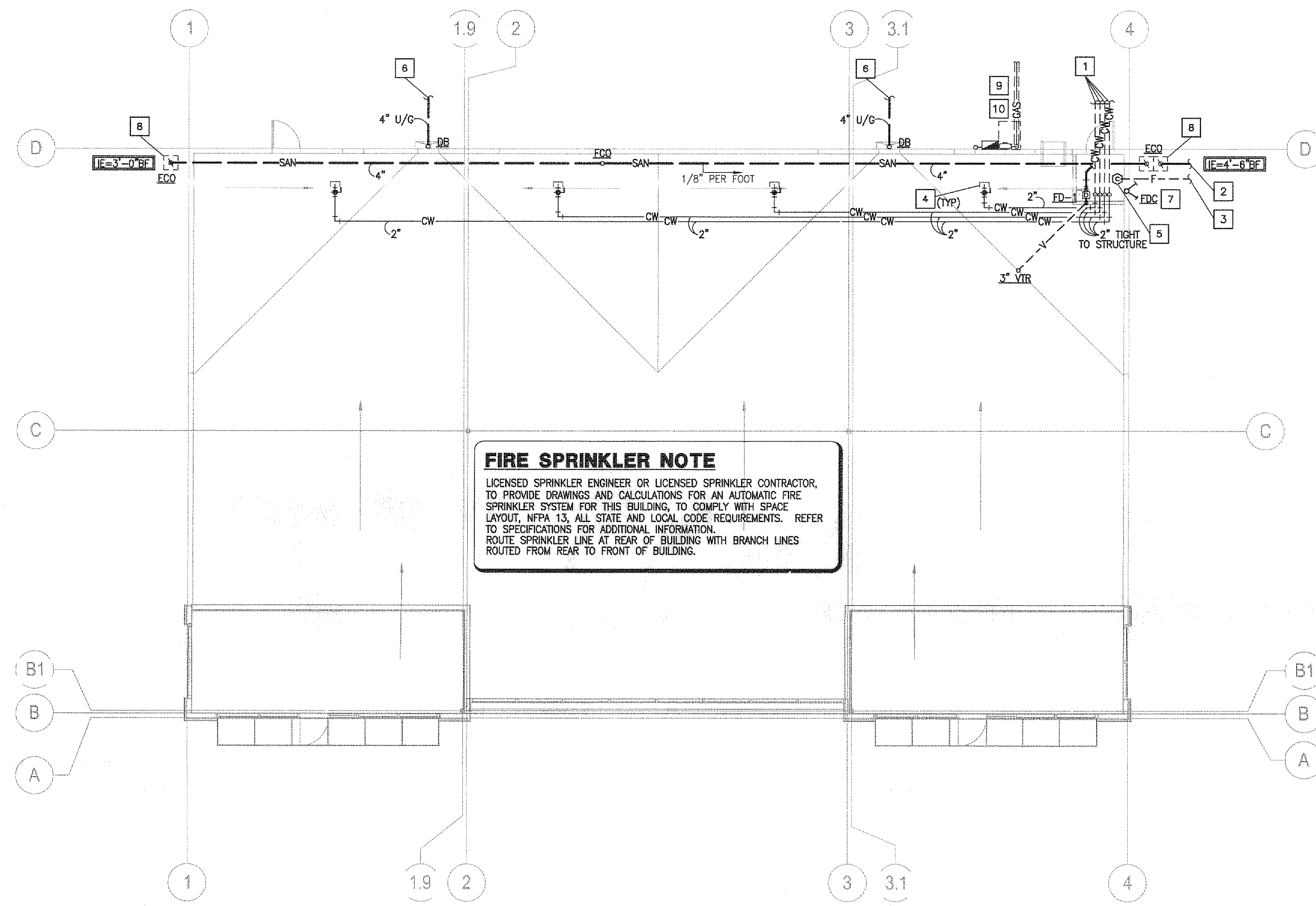
1 FLOOR PLAN - PLUMBING SCALE: 1/8"=1'-0"
