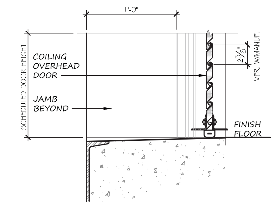
4 COILING OVERHEAD DOOR SILL DETAILS A4-8 SCALE: 3" = 1'-0"
