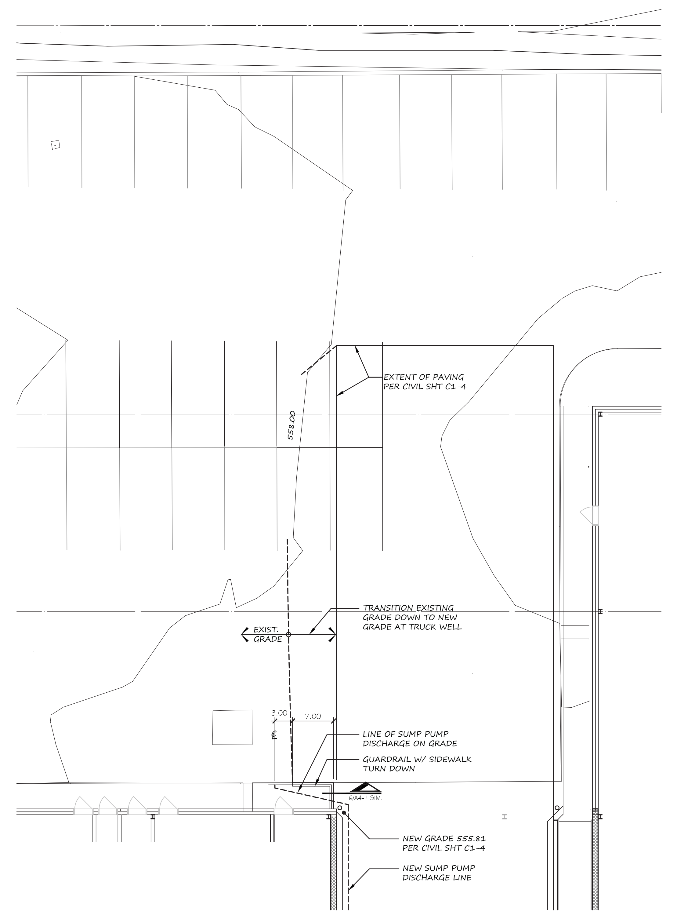
1 GRADING AT PETCO TRUCK WELL A4-8 SCALE: 1/8" = 1'-0"
