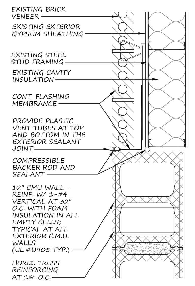
3 PLAN DETAIL A4-8 SCALE: 1 1/2" = 1'-0"
