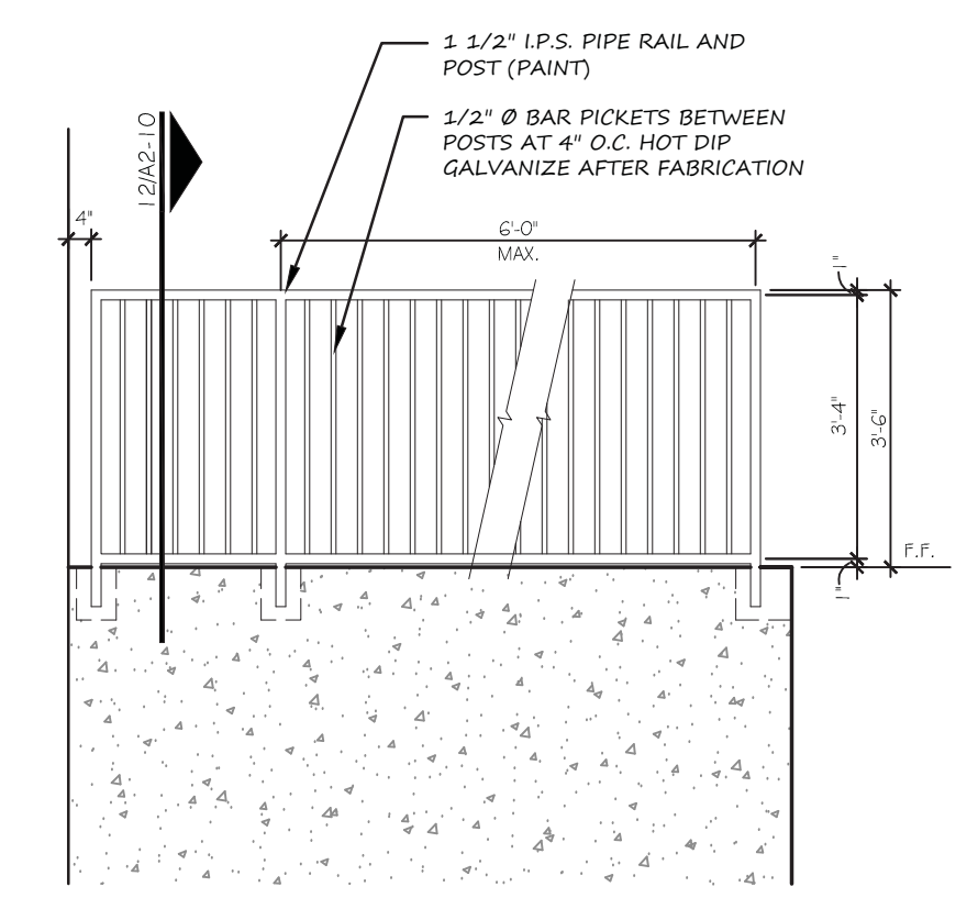
5 GUARD RAIL @ TRUCK DOCK A4-8 SCALE: 3/8" = 1'-0"
