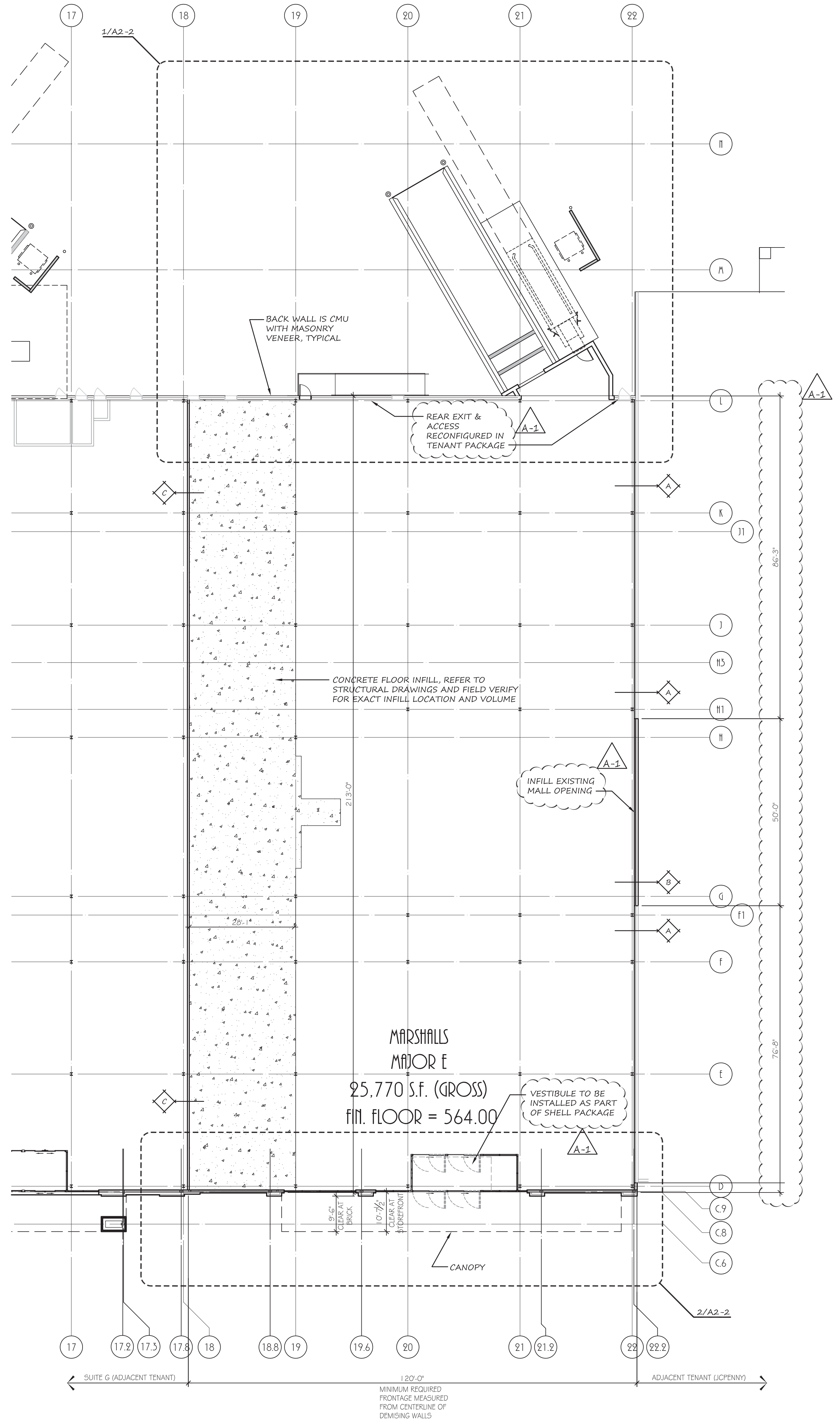
1 FLOOR PLAN A2-1 SCALE: 1/16" = 1'-0"
