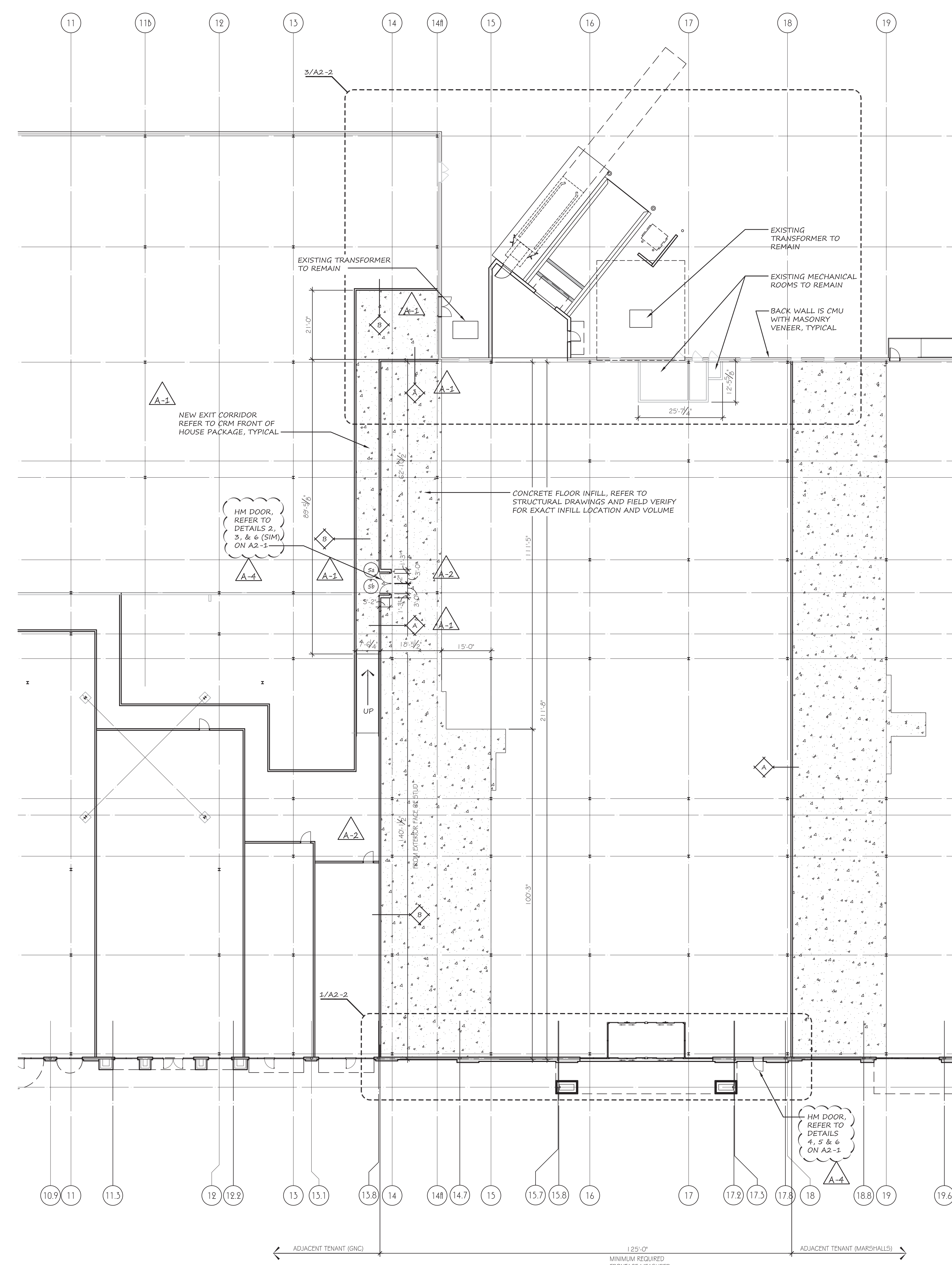
1 FLOOR PLAN A2-1 | SCALE: 1/16" = 1'-0"
