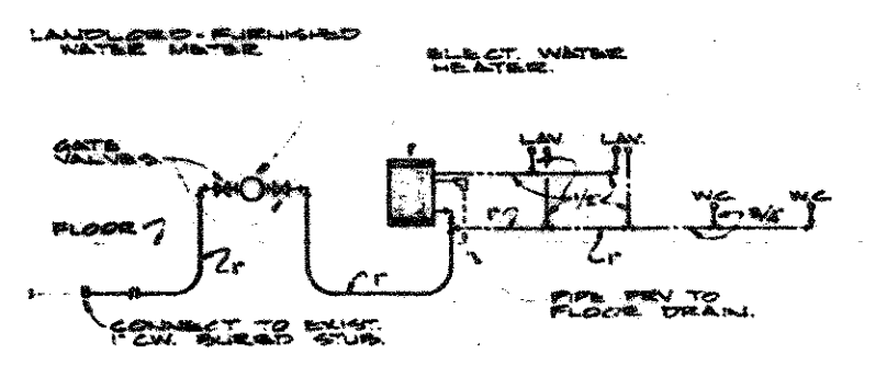
WATER PIPING SCHEMATIC NO SCALE
