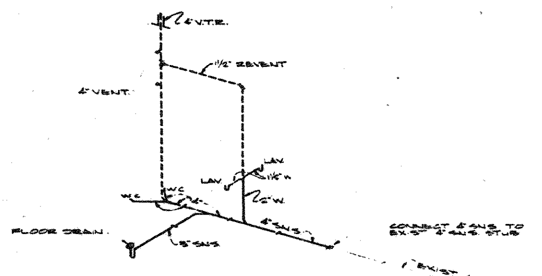
WATER PIPING SCHEMATIC NO SCALE
