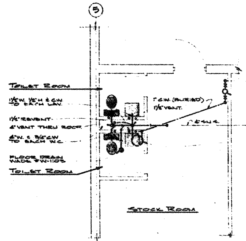
ENLARGED PLUMBING PLAN OF TOILET ROOMS SCALE: 1/4" = 1'-0"
