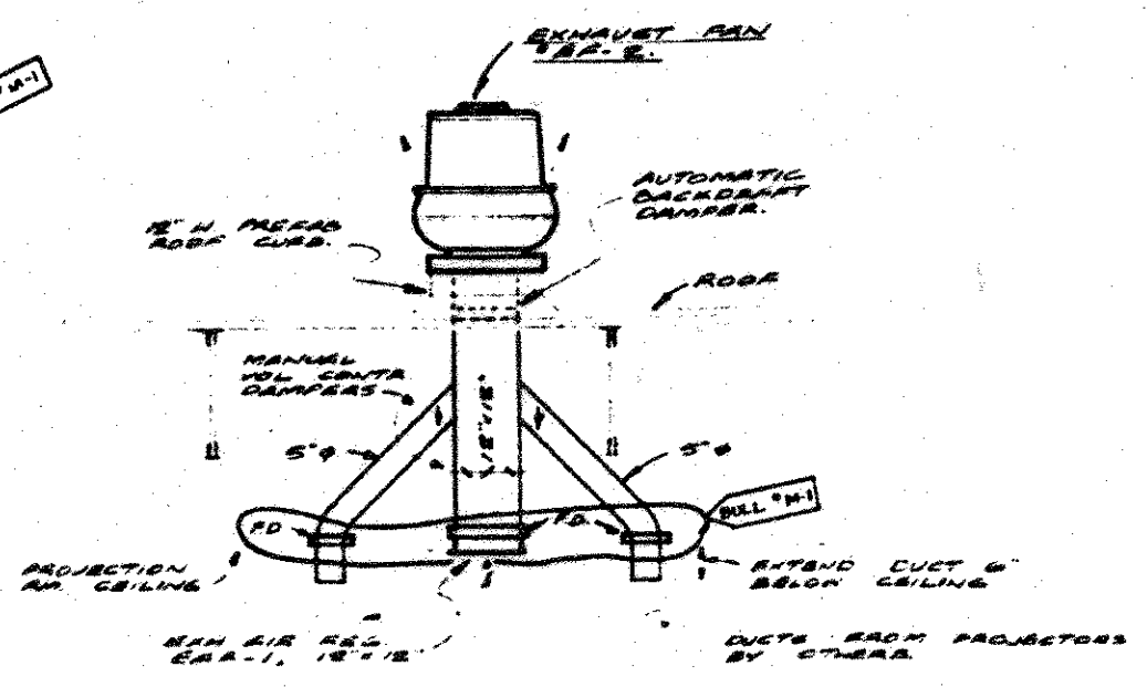
DETAIL SCALE 1/8\"/>
