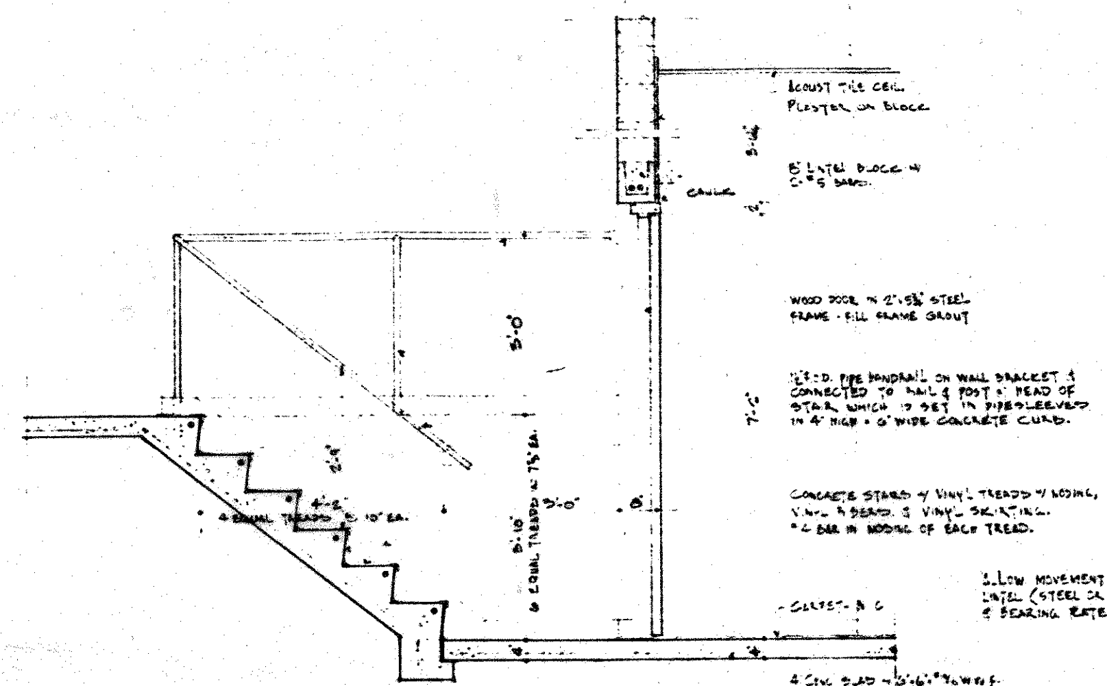
1 SECTION THRU STAIR ENTERING PROJECT ON ROOM SCALE 1/2" = 1'-0"
