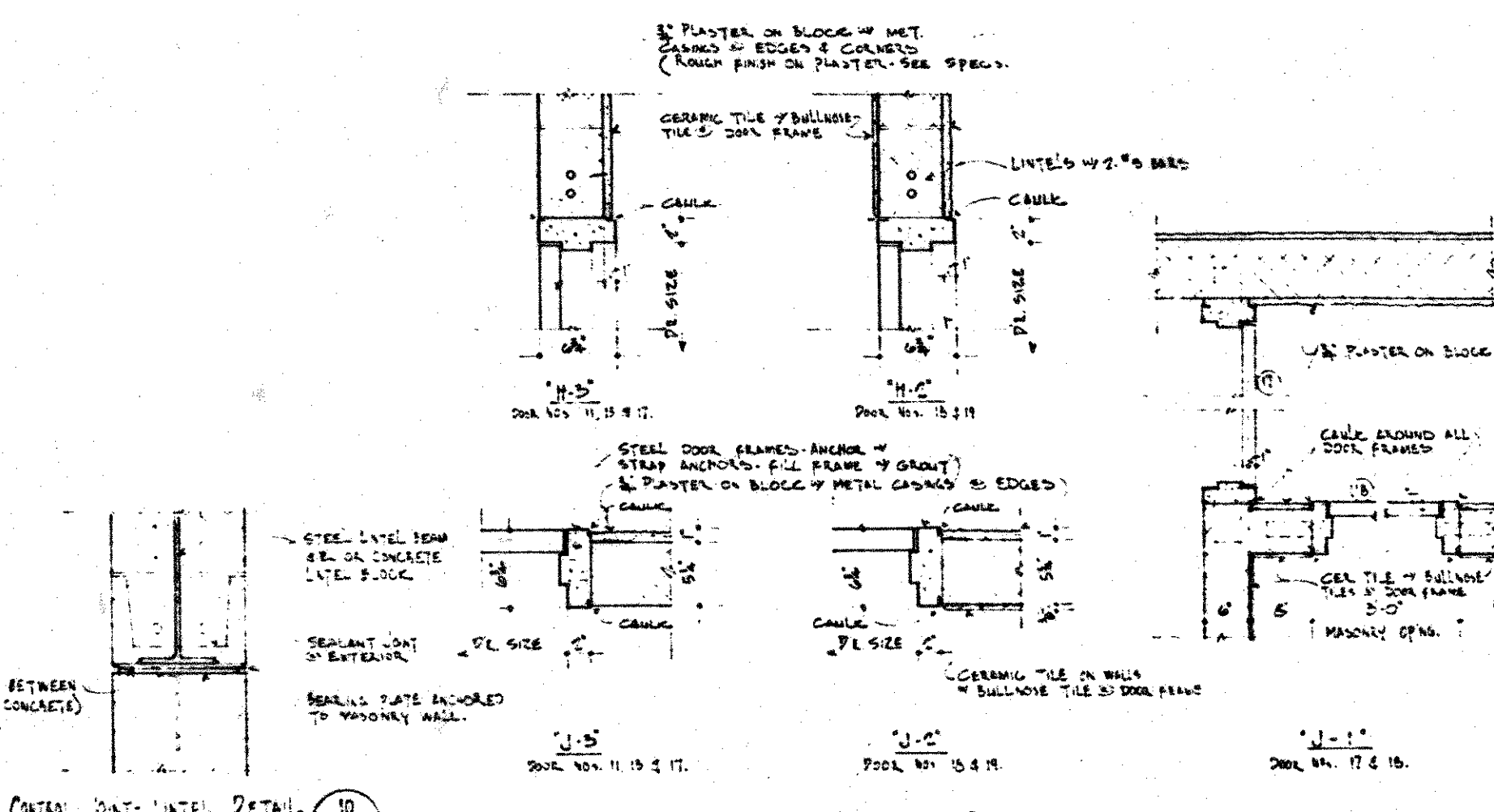
DOOR DETAILS SCALE 1/2" = 1'-0"
