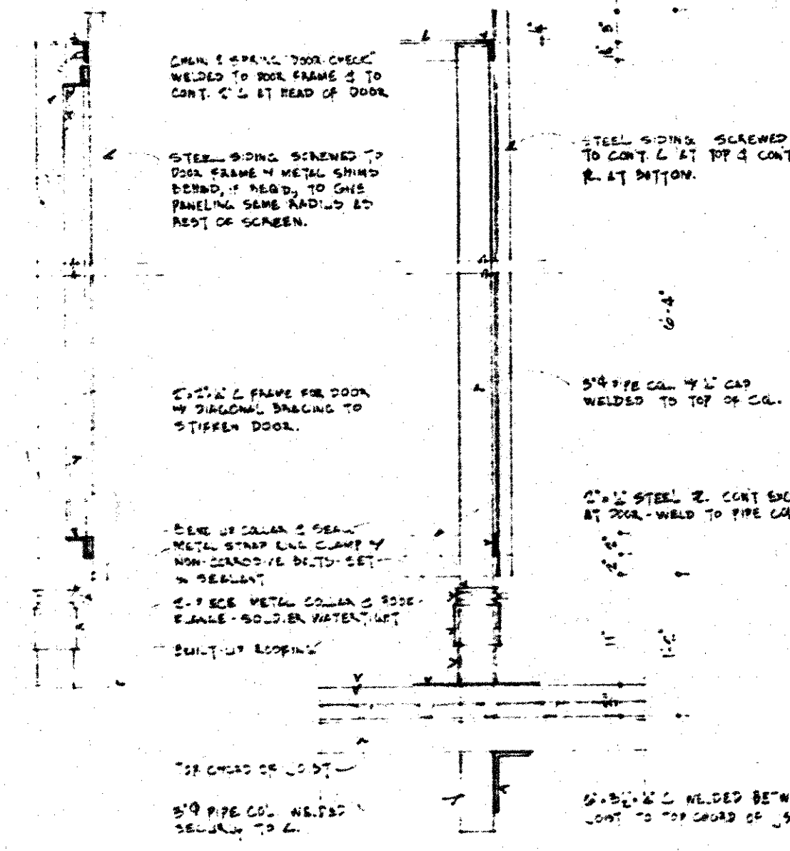
6 THRU ENCLOSURE DOOR SCALE 1/2" = 1'-0"
