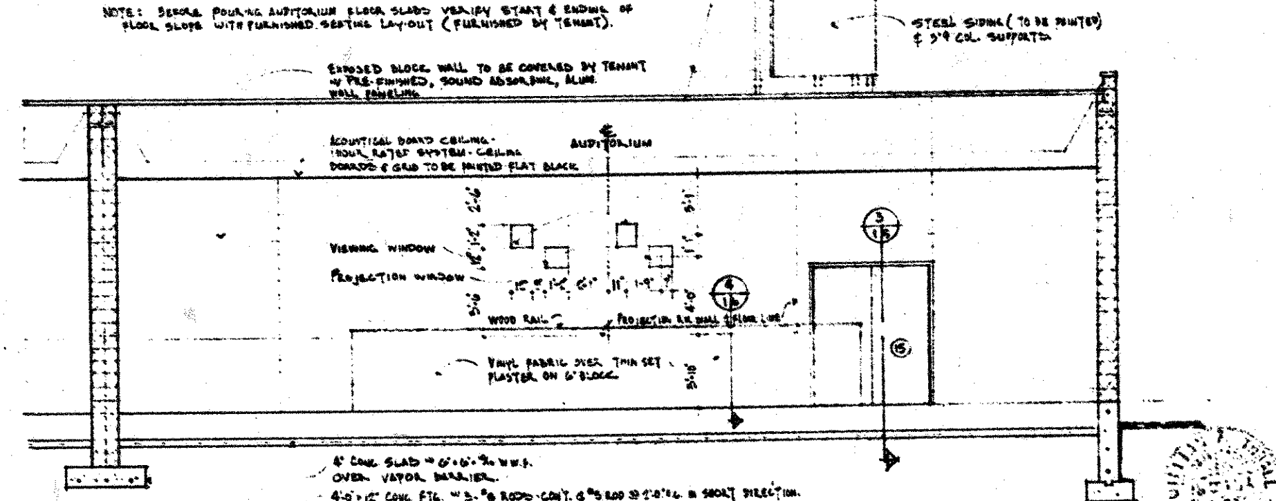
BUILDING CROSS SECTION 'B-1' SCALE 1/8" = 1'-0"
