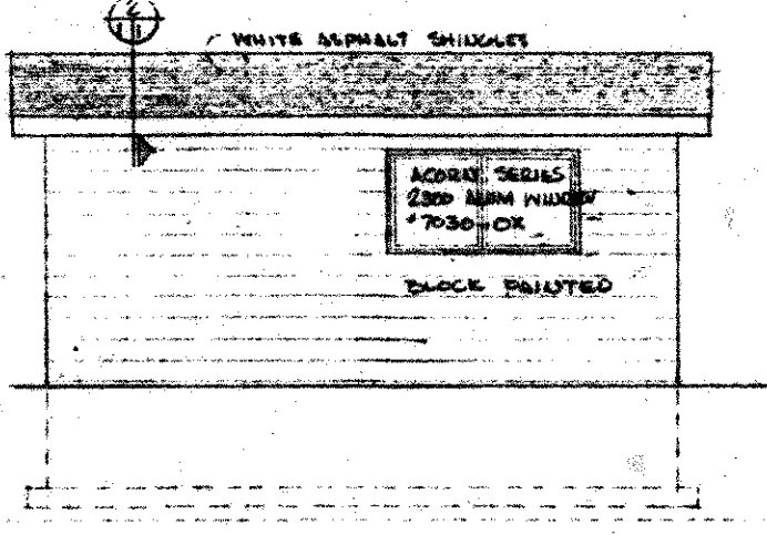
EAST ELEVATION SCALE: 1/2" = 1'-0"
