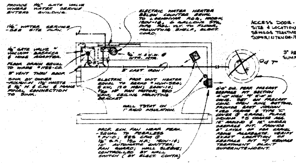
MECHANICAL PLAN SCALE: 1/4" = 1'-0"
