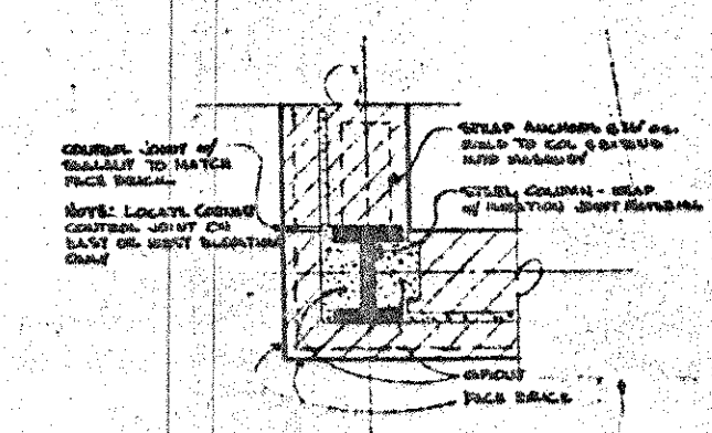
6 DETAIL OF CORNER COLUMN & CONTROL JOINT SCALE: 1/2" = 1'-0"
